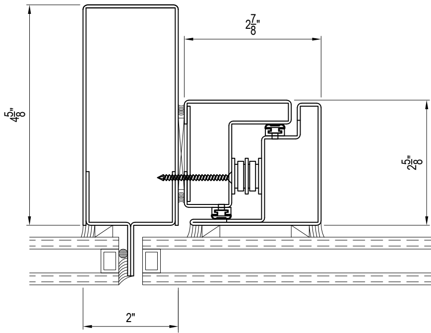
VENT SECTION
